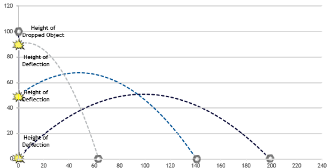
Figure 4: Dropped Object Maximum Deflection Distances
