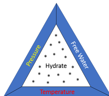
Figure 2: Hydrate Triangle.
