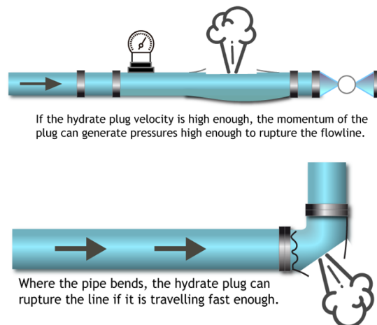
Figure 4. Impact and Overpressure Failures
