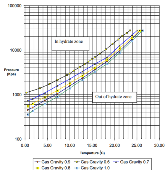
Figure 3. Pressure-Temperature Curves for Predicting Hydrate Formation
